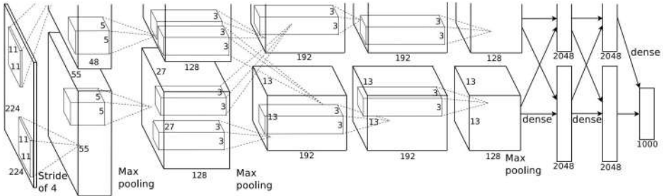
Figure 3: AlexNet architecture 9 . Please note that the input size in this figure is not 224x224 but 227x227
