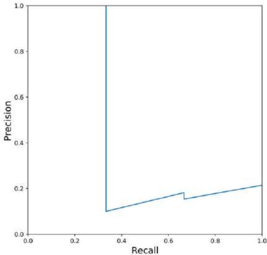
Figure 2: precision-recall curve
