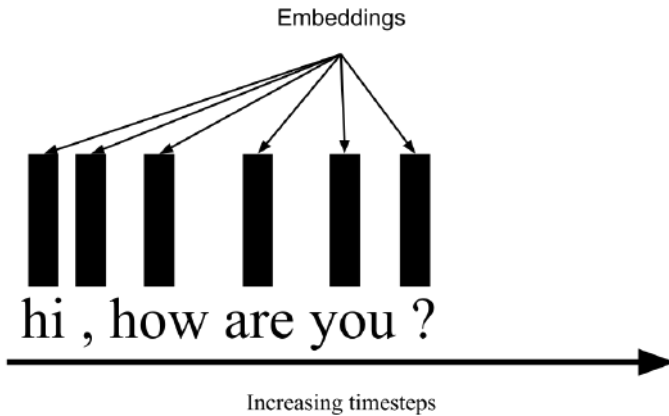
Figure 2: Representing tokens as embeddings and treating it as a time series
