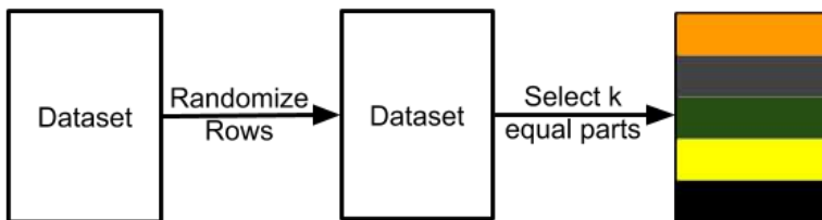
Figure 5: K-fold cross-validation
