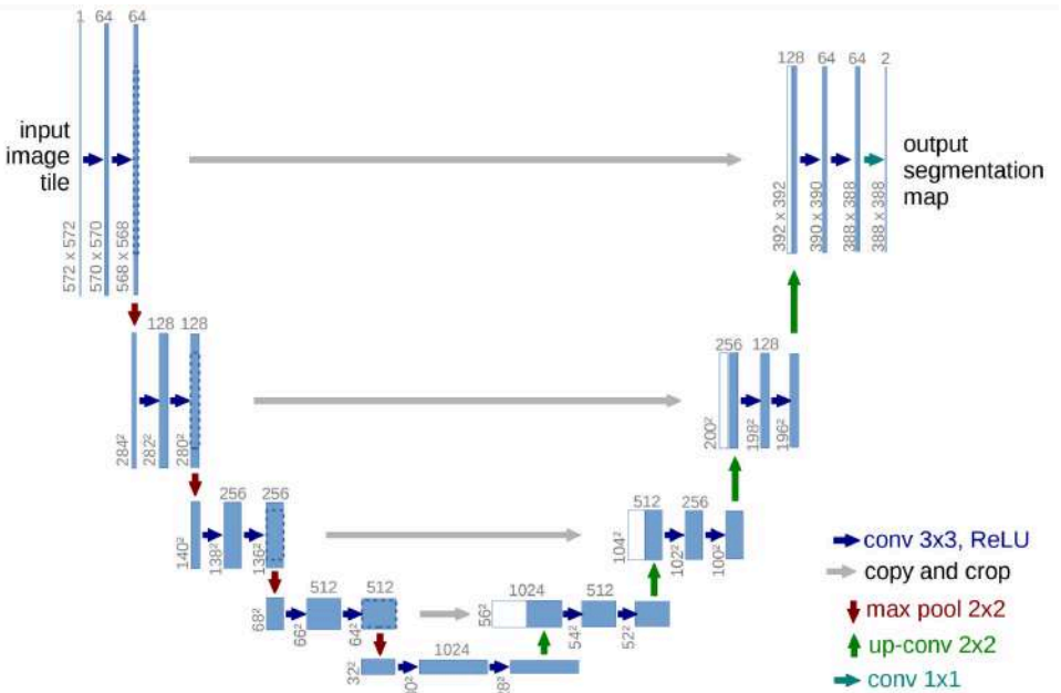
Figure 8: U-Net architecture 11 .
